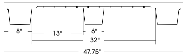
SHORT SIDE VIEW
