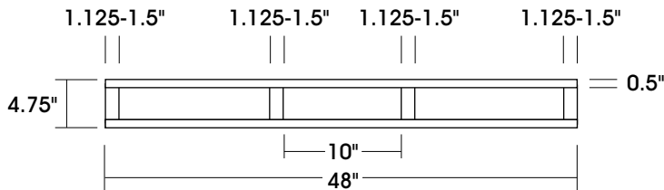
END VIEW
