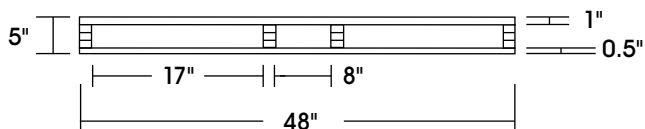
END VIEW
