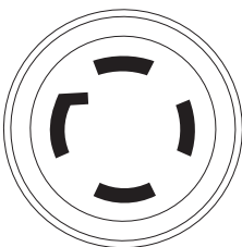
Figure 2-6. Prise 120/240 VCA, 30 A NEMA L14-30R
