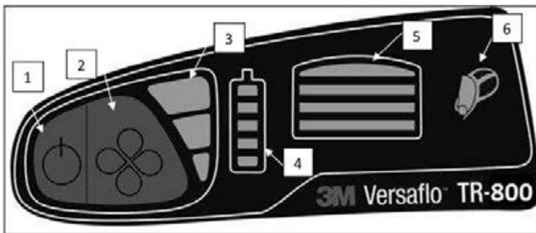
Figure 8: Motor/blower User Interface: (1) On/Off button, (2) Flow control button, (3) Airflow setting indicator, (4) Battery charge status level/alarm indicator, (5) Filter loading/alarm indicator, (6) Tight-fitting mode indicator
