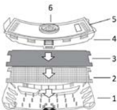
Figure 2: Attaching filter/cartridge to blower
