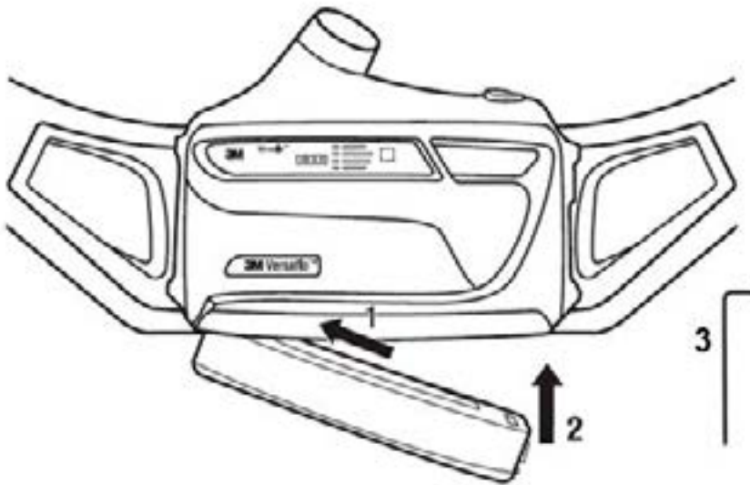
Figure 3: Installation de la pile
