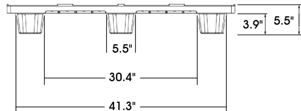
SHORT SIDE VIEW
