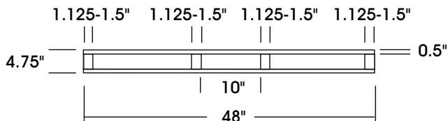
END VIEW
