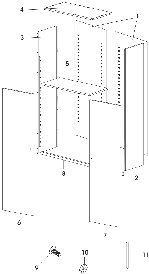
PRIMARY ASSEMBLY
