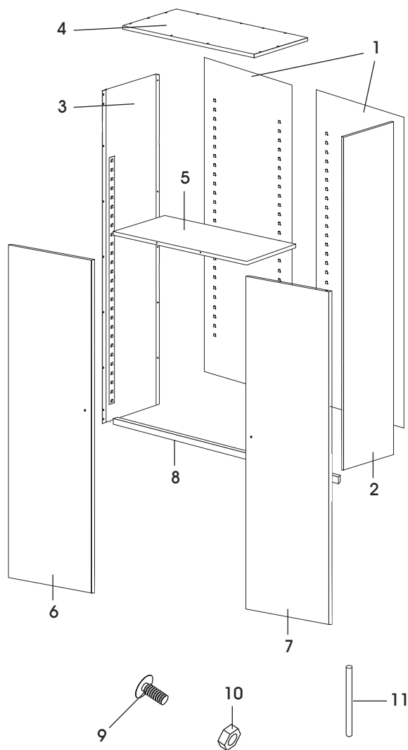
ENSEMBLE PRINCIPAL
