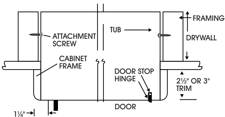
MOUNTING DIAGRAM (TOP VIEW)
