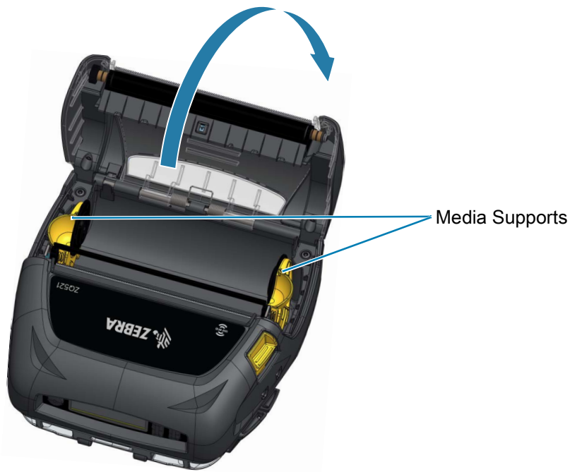
Figure 18 Opening the Media Cover
