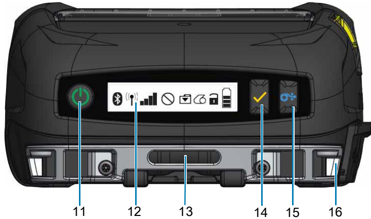
Figure 3 Printer Front Features
