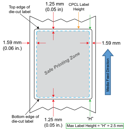
Figure 28 Journal Media
