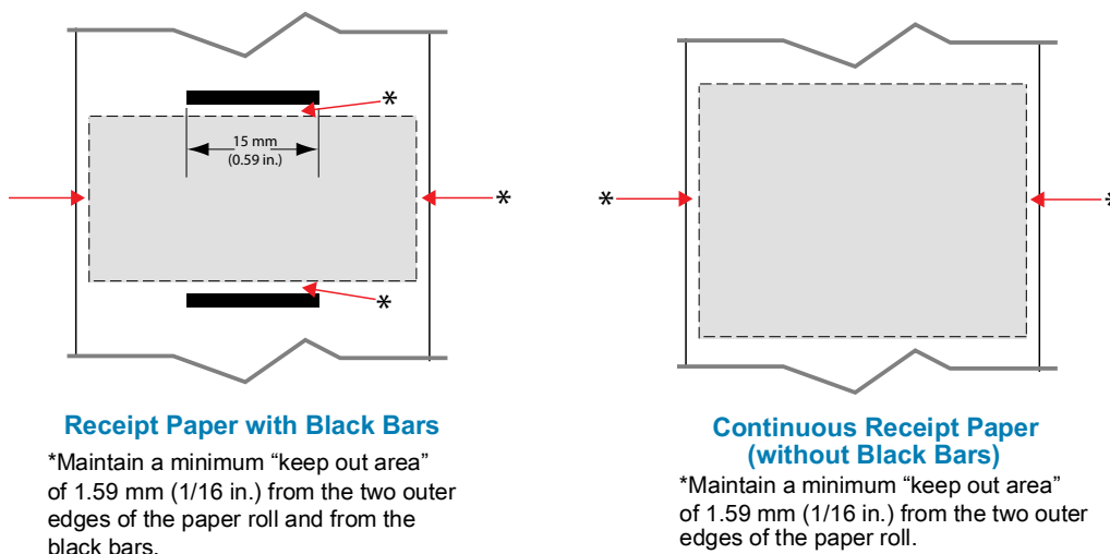
Figure 32 Keep Out Areas
