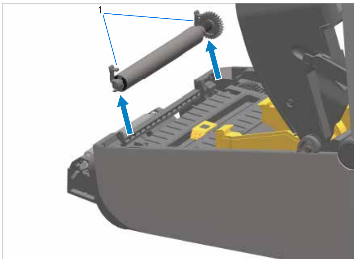
1 Platen bearings
