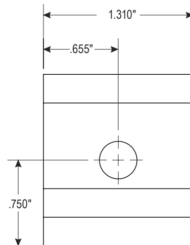
VISTA FRONTAL
