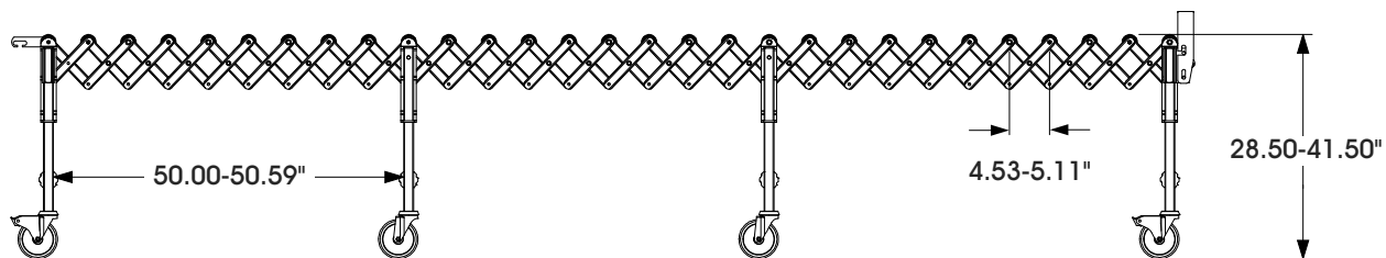
SIDE VIEW
