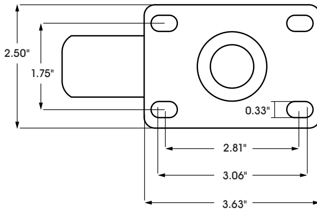
PLATE DIMENSIONS
