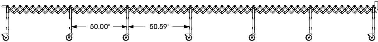
SIDE VIEW
