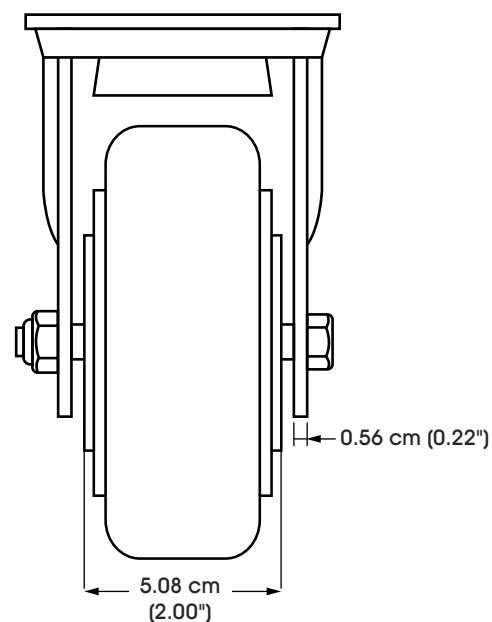
VISTA FRONTAL
