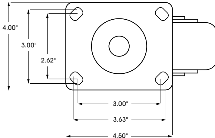
PLATE DIMENSIONS
