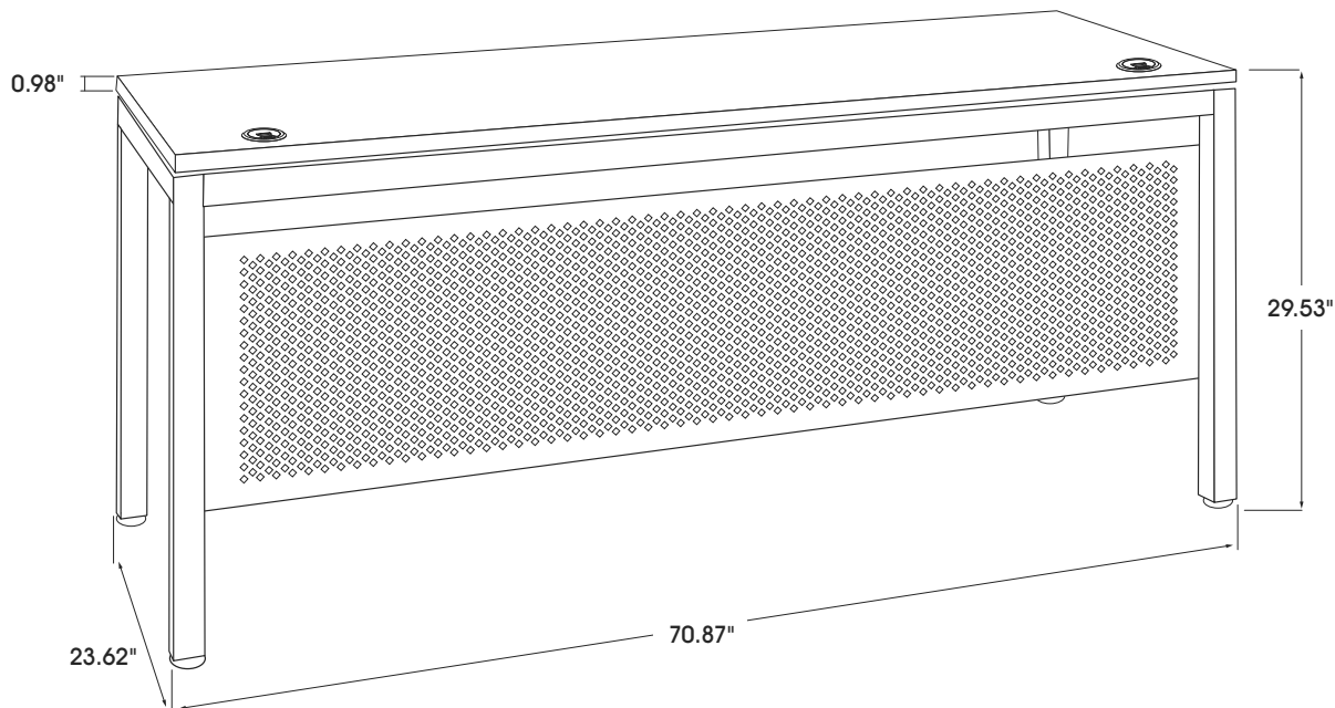
OUTSIDE VIEW
