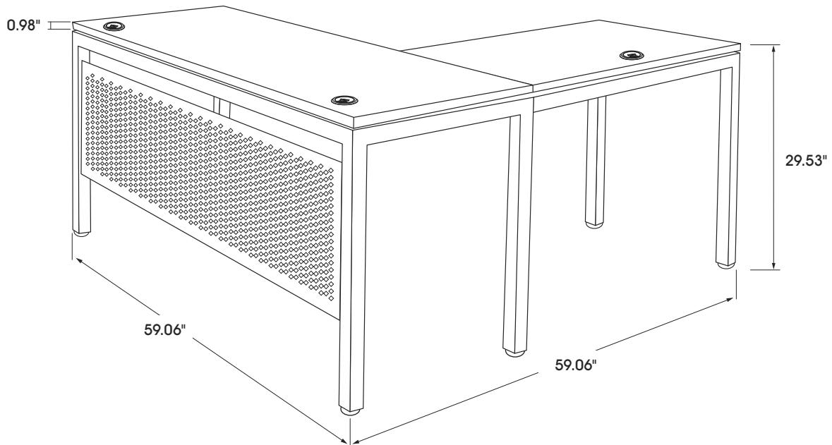
OUTSIDE VIEW
