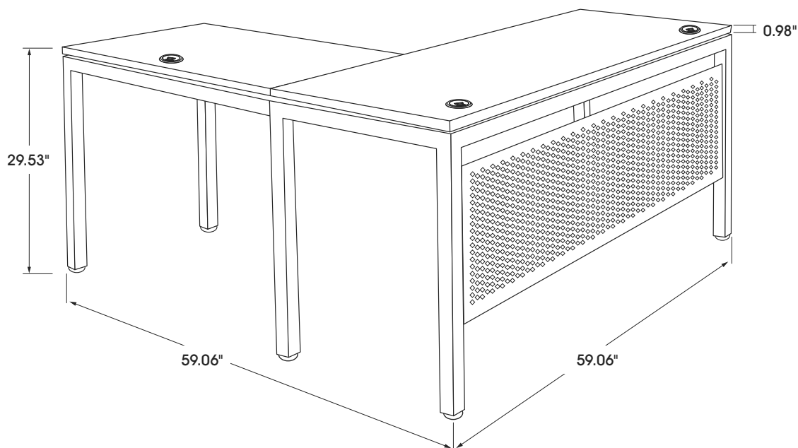
OUTSIDE VIEW
