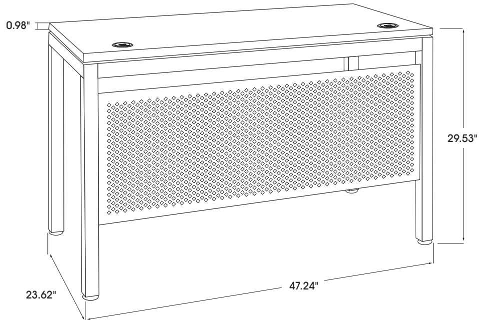
OUTSIDE VIEW
