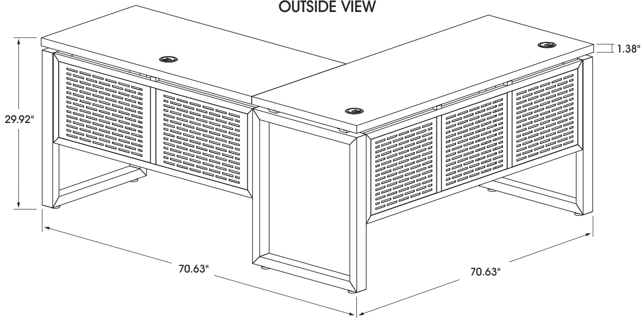
OUTSIDE VIEW
