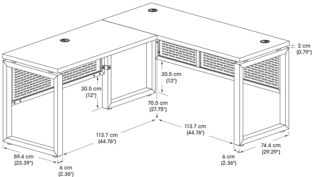
VISTA INTERIOR
