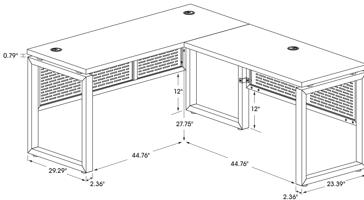
INSIDE VIEW
